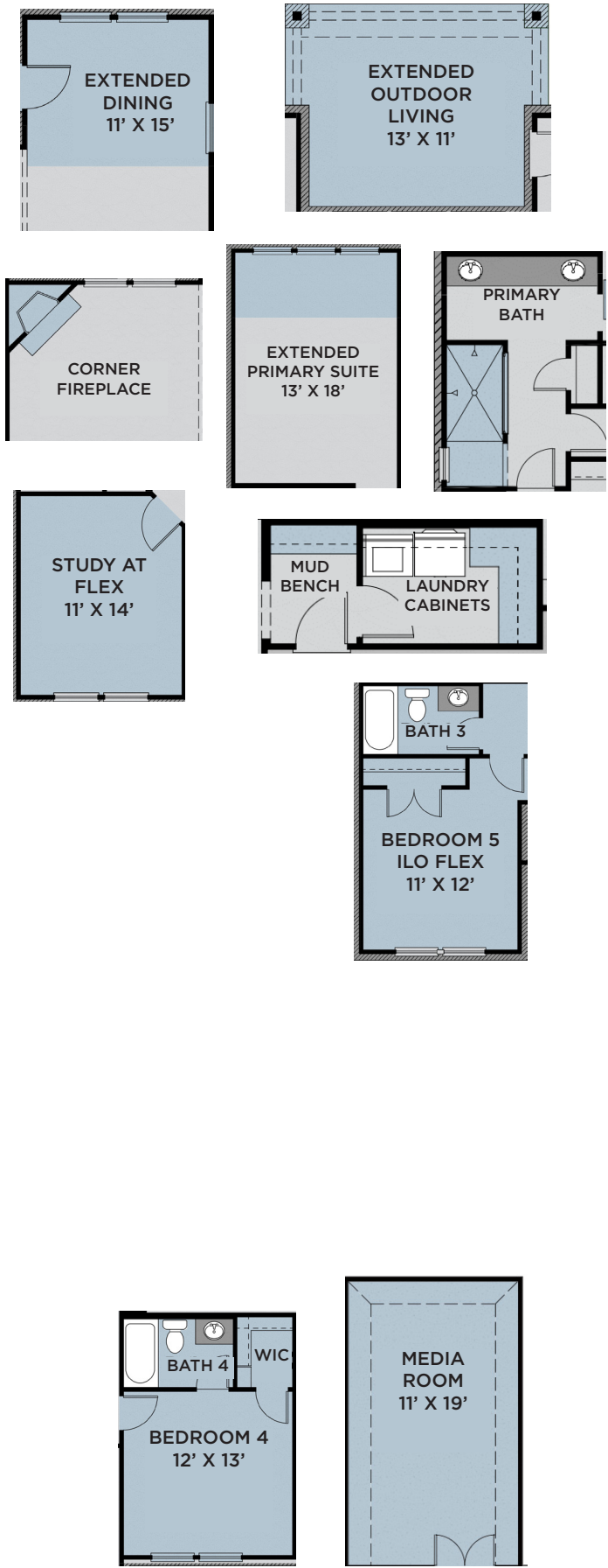
SECOND FLOOR
